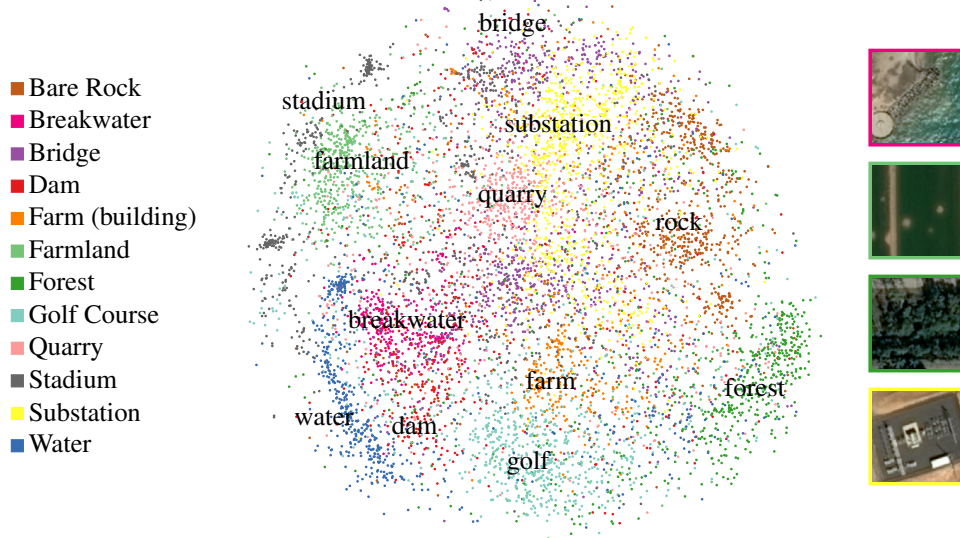
Figure 1: Learned representations of out-of-sample image scenes, visualized with PCA followed by t-SNE and colored by OpenStreetMap category. Without any labels, Contrastive Sensor Fusion has learned a representation that groups remote sensing images into semantically meaningful categories.
